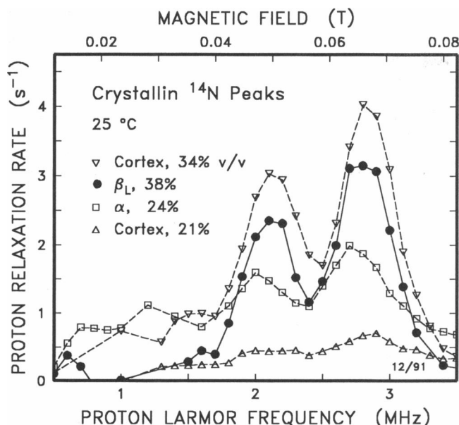
FIGURE 3 ^{14}\text{N} peaks (expanded) in the proton 1/T_1 NMRD profiles for 38% vol/vol \beta_L -crystallin, from the present work (●); for 24% bovine cortical \alpha -crystallin (□) (after 35); and 34% (▽) and 21% (Δ) calf cortical homogenate (after 32), all at 25°C.
