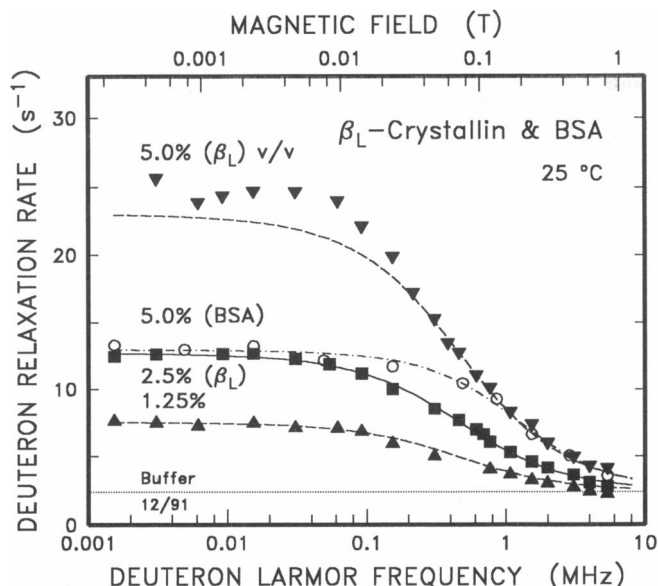
FIGURE 1 Deuteron 1/T_1 NMRD profiles of steer \beta_L -crystallin, 5% ( \nabla ), 2.5% ( \blacksquare ), and 1.25% ( \blacktriangle ) vol/vol, and 5% vol/vol bovine serum albumin (BSA) ( \circ ), at 25°C. The solid curve through the data points for the 2.5% sample, and the dot-dashed curve through the BSA data, derive from least squares comparisons of the data with the Cole-Cole expression, Eq. 1. The dashed curves associated with the 1.25 and 5% \beta_L -crystallin profiles were obtained by scaling the solid curve by the factors 0.5 and 2, respectively (correcting appropriately for the buffer background indicated). The excellent agreement with the 1.25% data indicates no change in solute association between the two concentrations; the \sim 12\% difference for the 5% data suggests a small, but not significant, increase in association at the higher concentration. The more than four-fold higher value inflection field of the (68 kD) BSA profile indicates that the molecular weight of \beta_L -crystallin, assuming it is compact and reasonably spherical, is greater than that of BSA by this factor (see text).
